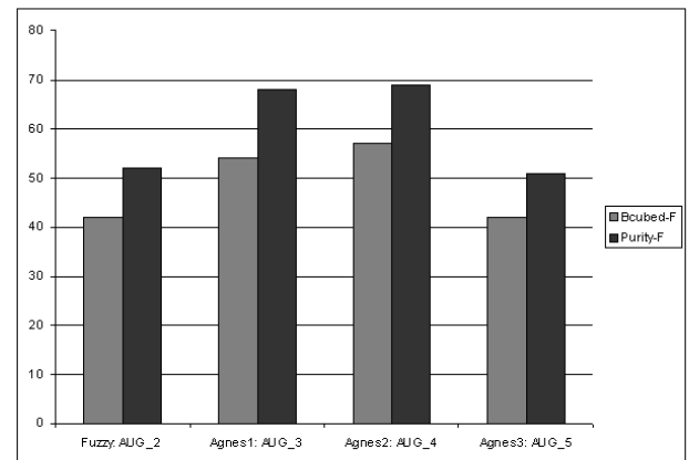
Figure 3: Results for Fuzzy and hierarchical clustering (Agnes) on three different clustering thresholds for the second WePS testbed.
