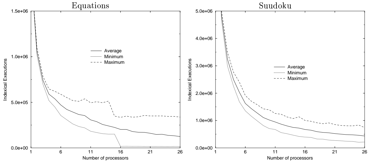
Figure 9: Indexical executions per processor (Ready Set balance / Immediate Broadcast)
